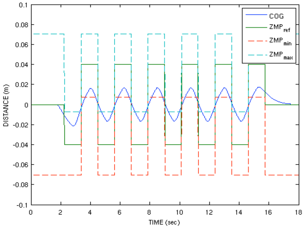
Fig. 6. Trajectory of the COG and the ZMP reference.
