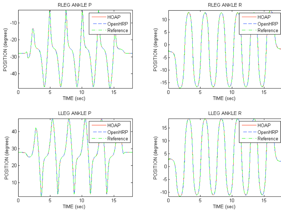
Fig. 13. Trajectories for the 2 DOF of the right and left ankles, both in OpenHRP3 and HOAP-3.
