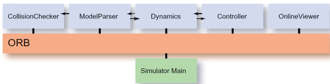
Fig. 1 OpenHRP3 functions.
