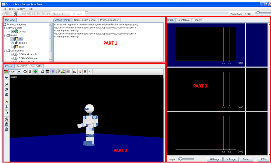
Fig. 2. OpenHRP interface.
