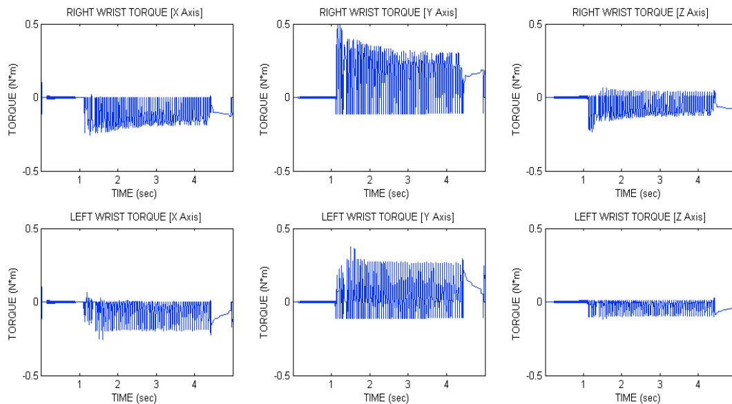
Fig. 16. Torques of right (up) and left (down) wrists during the touching motion.
