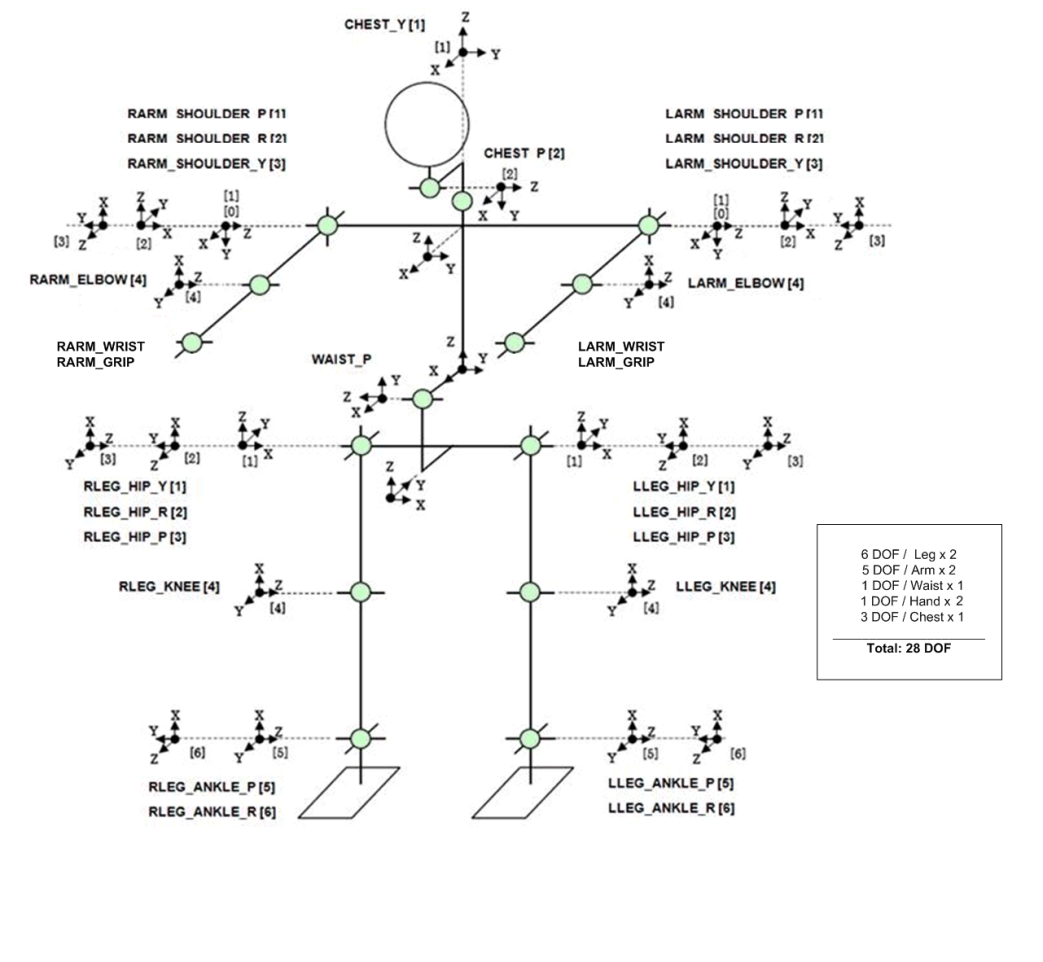
Fig. 3. Distribution of DOF in HOAP-3.
