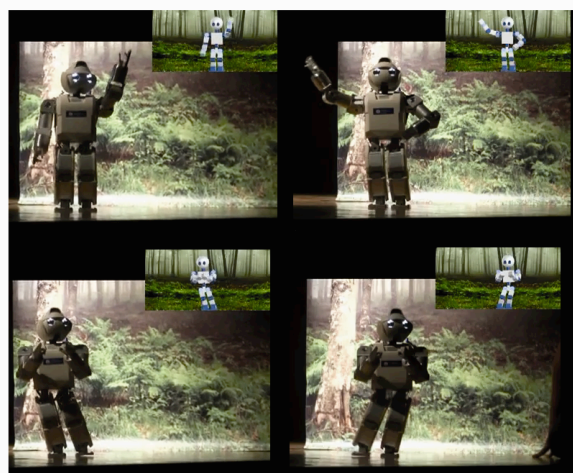
Fig. 14. HOAP-3 dancing in an exhibition during 3 minutes. The simulation is run and shown in a top window during the performance.
