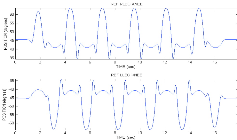
Fig. 8. Trajectories for the 1 DOF of the right and left knees, respectively.
