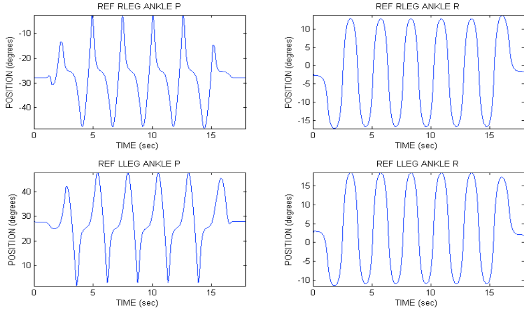
Fig. 9. Trajectories for the 2 DOF of the right and left ankles, respectively.
