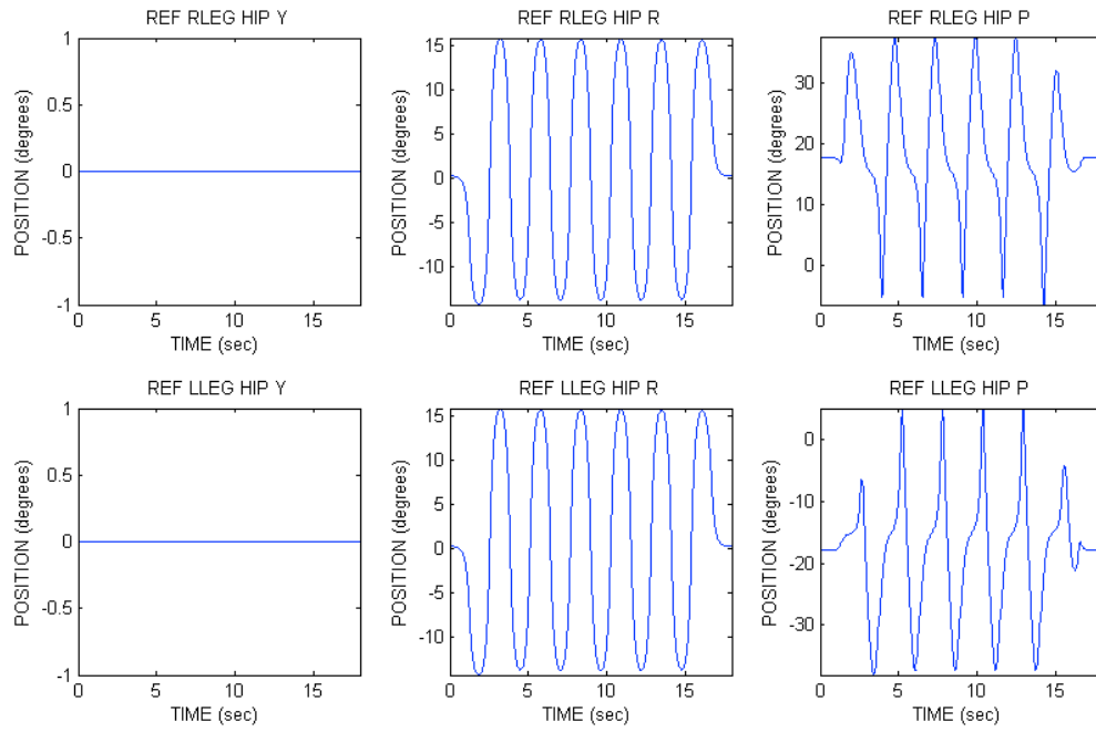
Fig. 7. Trajectories for the 3 DOF of the right and left hips, respectively.
