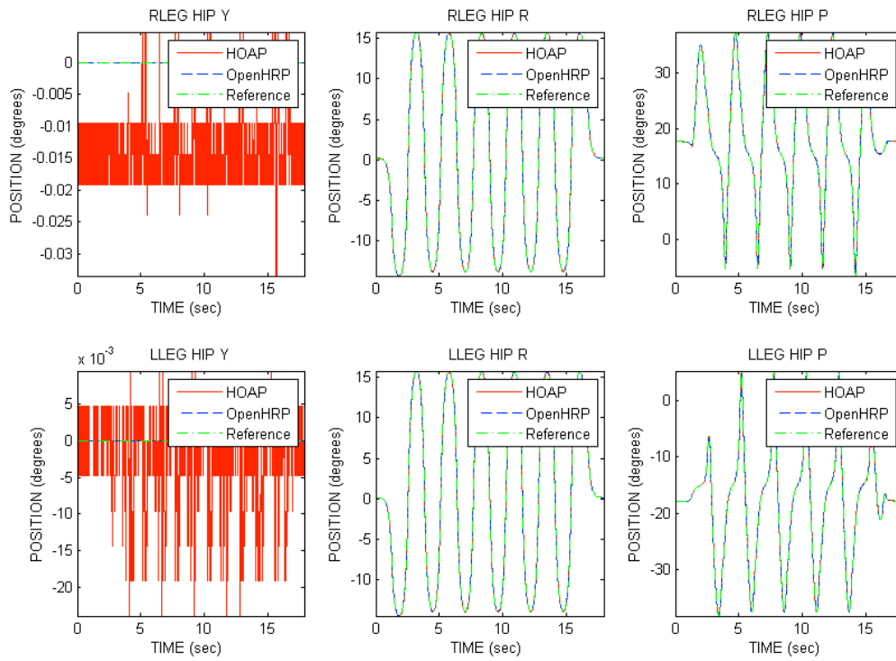
Fig. 11. Trajectories for the 3 DOF of the right and left hips, both in OpenHRP3 and HOAP-3.
