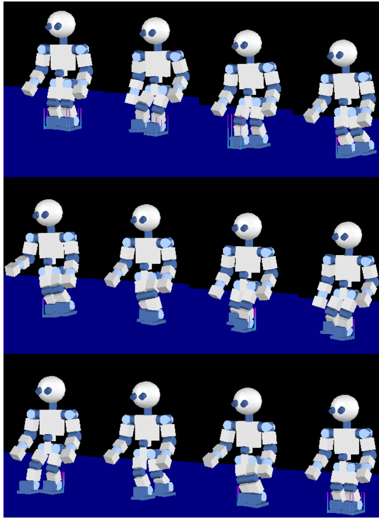
Fig. 10. Sequence of motions for HOAP-3 during a step.
